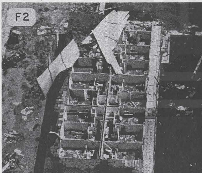
An example of Fujita-scale damage. Corresponding windspeeds are F0 (less than 73 mph), F1 (73-112), F2 (113-157), F3 (158-206), F4 (207-260), F5 (261 mph or higher).
